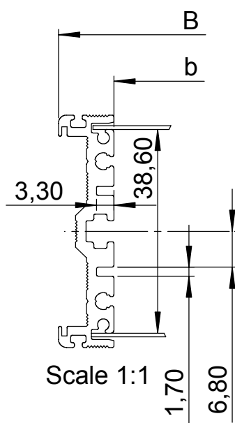
Side panel(broken out view)
